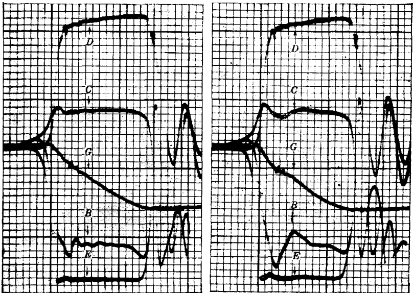
(a) Six-section pulse-forming network with Z_N = 1000 ohms.
